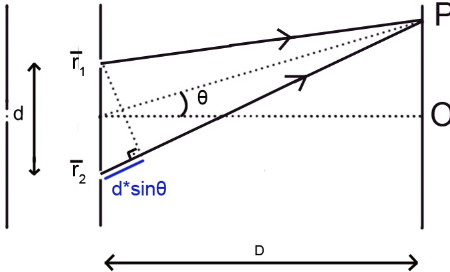
FIGURE 1 – Double fente de Young
