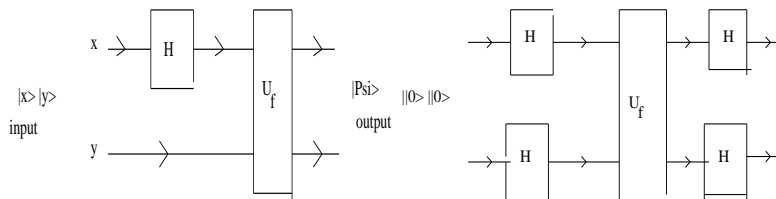
Figure 12.2 Deutsch illustration of quantum parallelism
