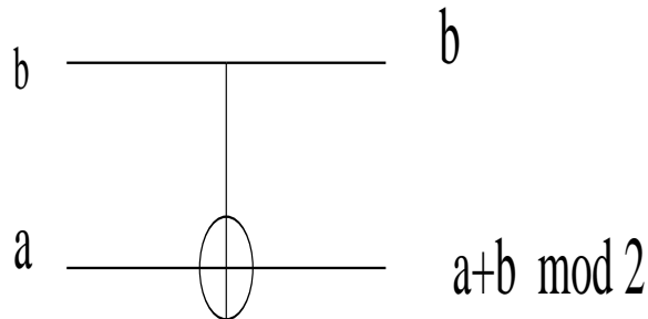
Figure 12.3 CNOT gate
