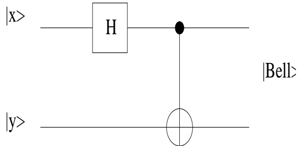
Figure 7.4 Machine for producing Bell states
