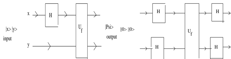
Figure 7.2 Deutsch illustration of quantum parallelism
