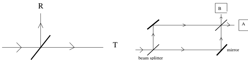
Figure 7.1 beam splitter and Mach-Zehnder interferometer
