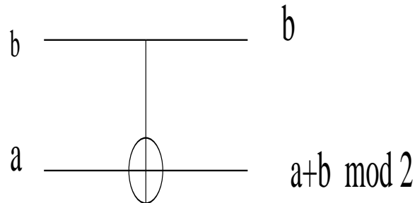
Figure 13.3 CNOT gate
