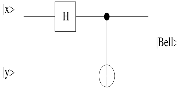
Figure 13.4 Machine for producing Bell states
