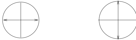
Figure 3.2 orientations of polarizer for preparation of photons in Z basis
