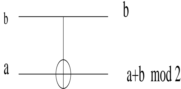
Figure 5.3 CNOT gate
