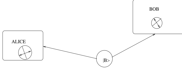
Figure 4.2 Alice and Bob share an entangled pair.
