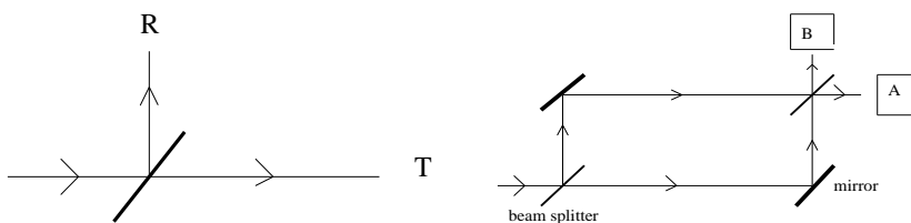
Figure 5.1 beam splitter and Mach-Zehnder interferometer
