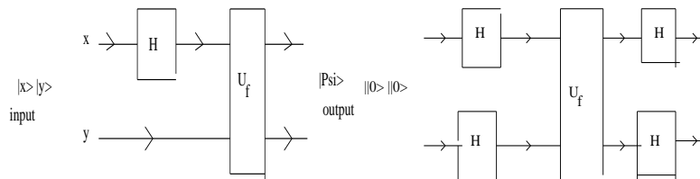
Figure 9.2 Deutsch illustration of quantum parallelism
