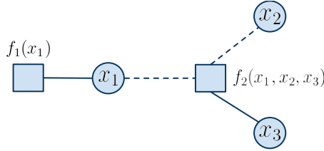
Figure 9.1 Factor graph of the equation F = x_1 \wedge (\bar{x}_1 \vee \bar{x}_2 \vee x_3)
