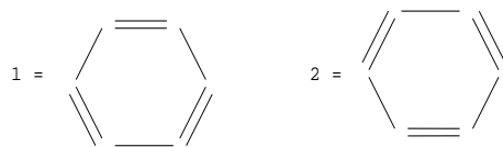
Figure 1.7: possible arrangements of chemical bonds
