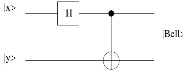
Figure 1: Machine for producing Bell states
