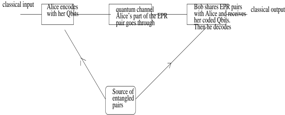
Figure 9.3: Alice and Bob share entanglement in order to communicate
