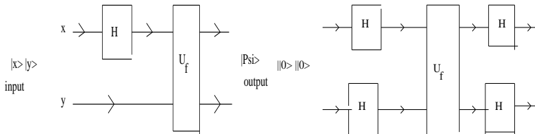
Figure 2: Deutsch illustration of quantum parallelism
